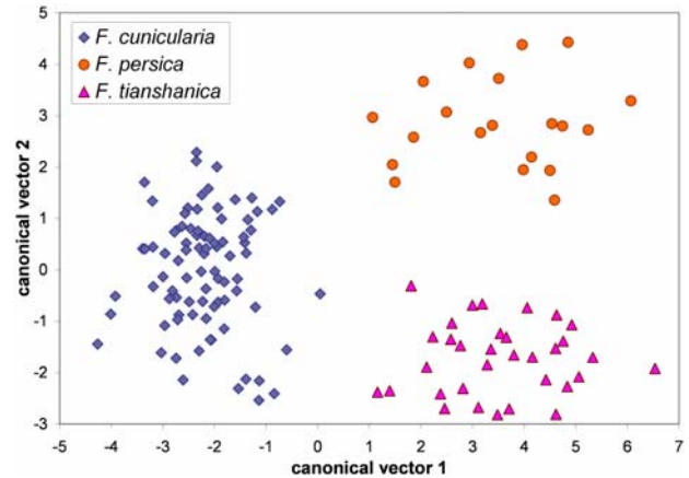
Fig. 17: Discriminant analysis of worker nest samples considering 14 characters of F. cunicularia , F. persica sp.n. and F. tianshanica sp.n.
