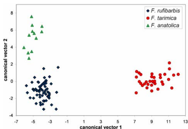
Fig. 15: Discriminant analysis of worker nest samples considering 14 characters of F. rufibarbis , F. tarimica sp.n. and F. anatolica sp.n.
