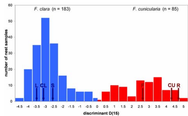
Fig. 14: Discriminant analysis of worker nest samples considering 15 characters of the Palaearctic population of F. clara and F. cunicularia . Position of type samples shown by arrows: CL – F. clara , L – F. lusatica , CU – F. cunicularia , R – F. fusca var. rubescens , F – F. cunicularia fuscoidea , S – F. rufibarbis var. sinae .
